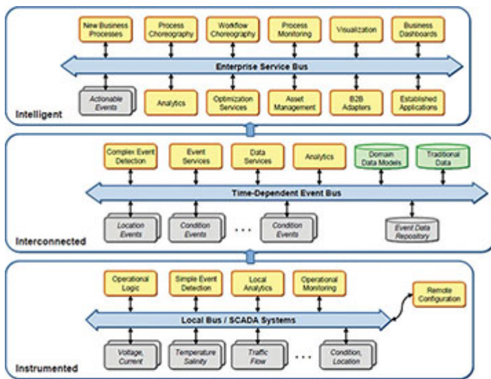
Fig. No.4 The architecture of a Smart ICT Platform
